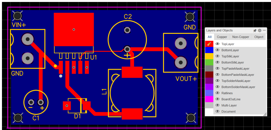
Image 1 – PCB Layout (Top View, Copper + Silkscreen)
