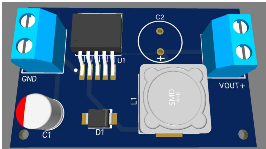
Image 3 – 3D View Top layer
